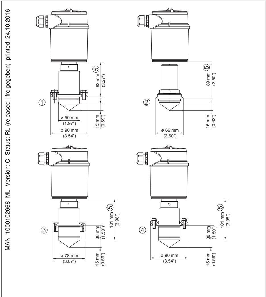
Fig. 39: LEVEL TRANSMITTER 8138, hygienic fitting 1
