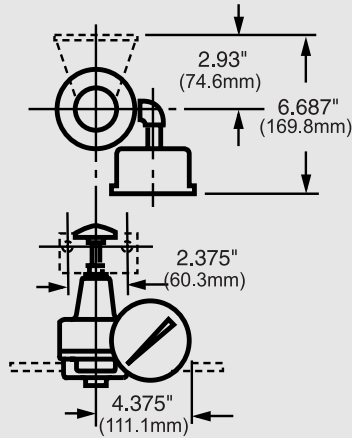
Pipe or Bracket-Mounted with Gauge
