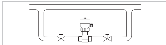
Fig. 7.2: Installation of the bypass fitting
