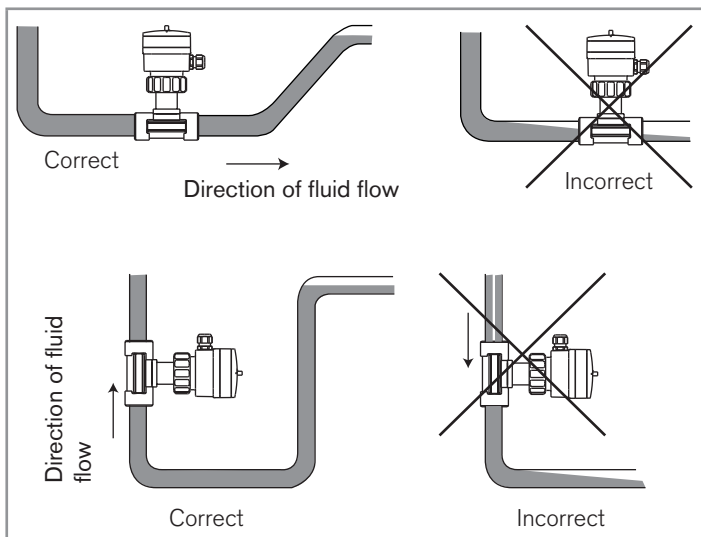
Fig. 7.6 Additional recommendations on installation
