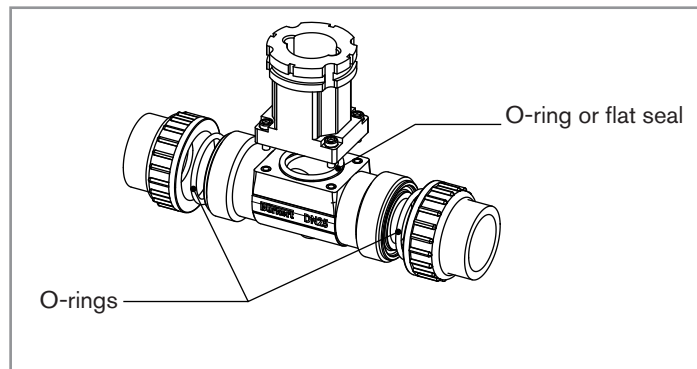
Fig. 11.4: Seals for a T-fitting with true union connection
