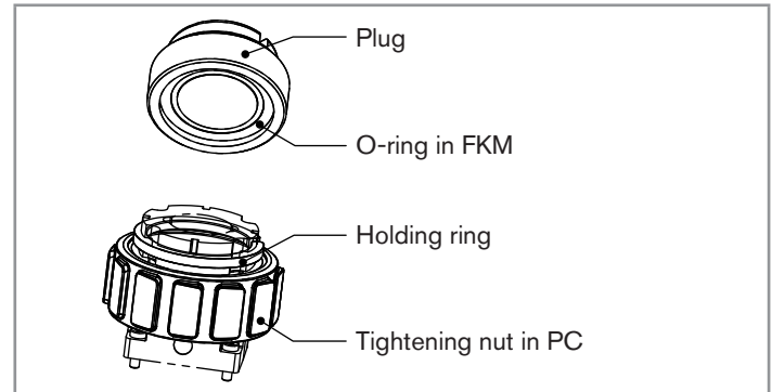
Fig. 11.3: Plug with O-ring, tightening nut and holding ring
