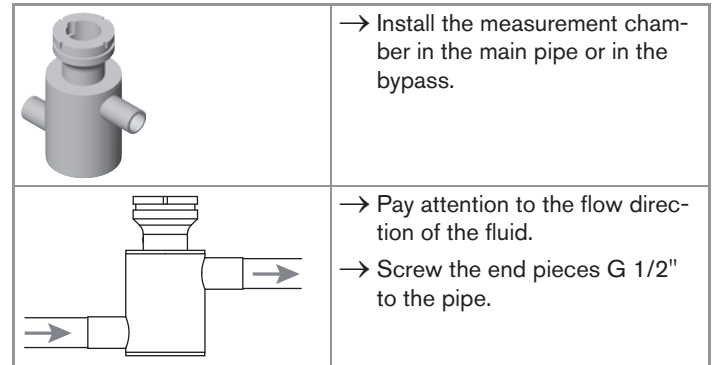
Fig. 7.13: Installing the measurement chamber
