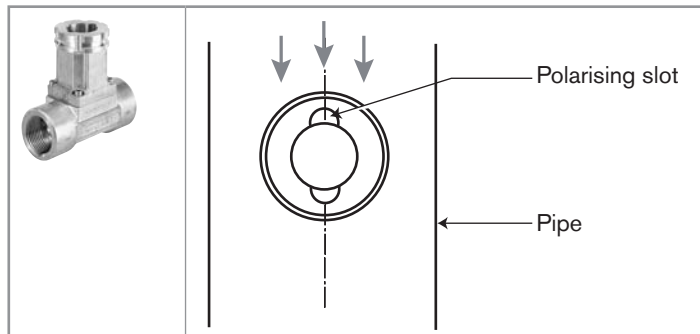
Fig. 7.7: Installing a T-fitting
