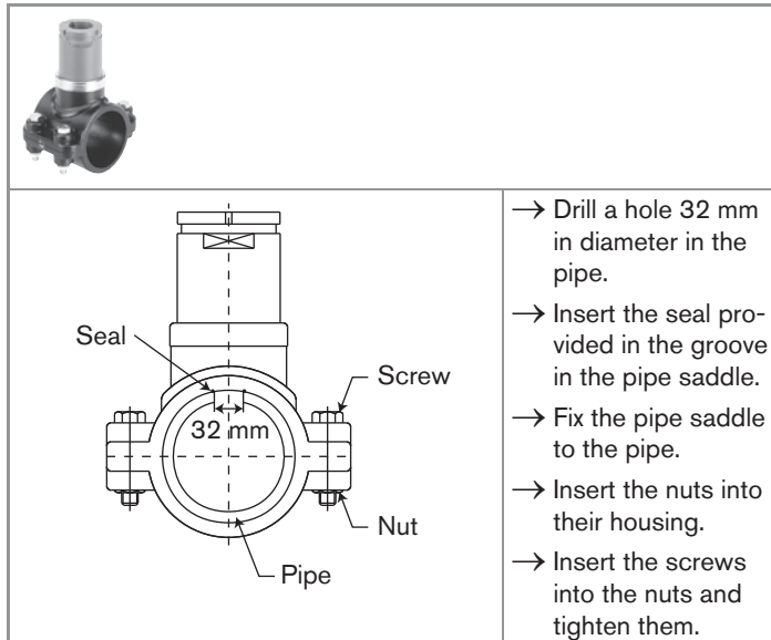
Fig. 7.8: Installing a fitting with pipe saddle
