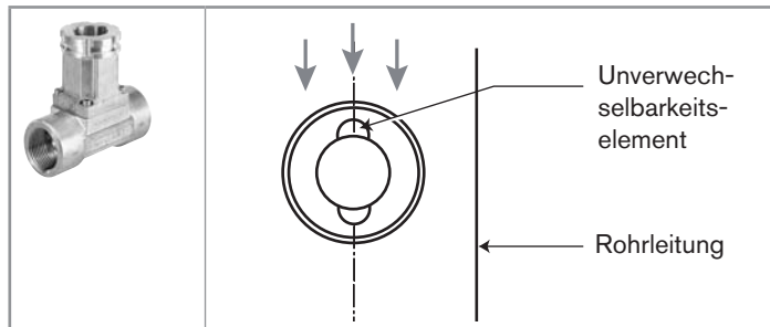
Abb. 7.7: Installation eines T-Fittings
