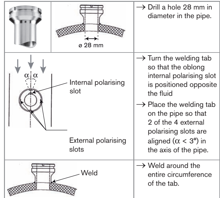
Fig. 7.9: Installing a welding tab
