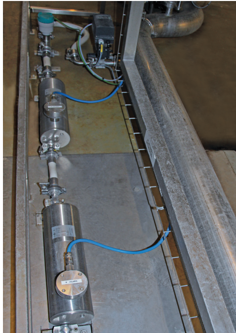
The field test setup, consisting of two existing Siemens Coriolis meters and the new SITRANS FC430.
