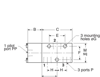
Pilot Operated - Pilot Return 2326B11-VR2B
