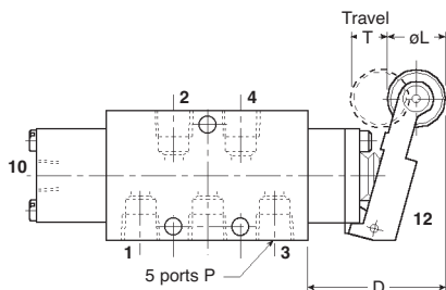
Roller/Lever Operated 2526M28-VR2B
