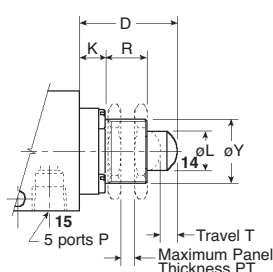
Plunger Operated 2526M26-VR2B, 2526M265VR2B
