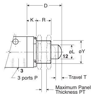
Plunger Operated 2326M26-VR2B, 2326M265VR2B
