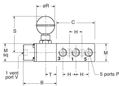
Pilot Operated - Spring Return with Latch Lock 2526M212VR2B, 2526M218VR2B
