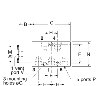
Pilot Operated - Spring Return 2526M21-VR2B
