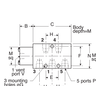
Pilot Operated - Pilot Return 2526B11-VR2B
