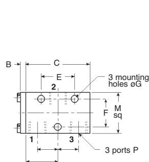
Pilot Operated - Spring Return 2326M21-VR2B
